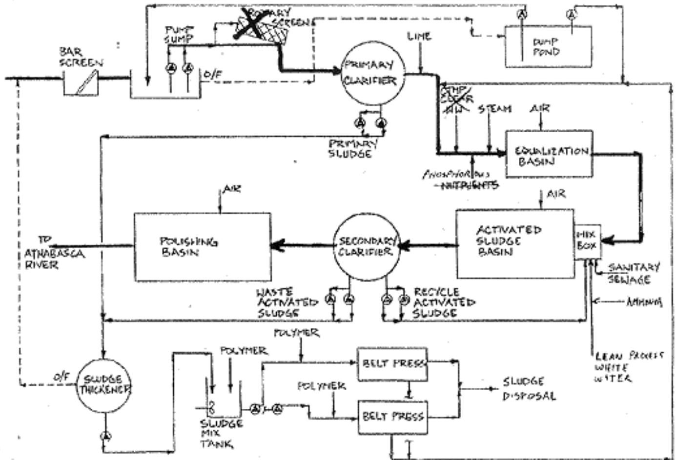
FIGURE 1: ANC WASTEWATER TREATMENT PLANT
